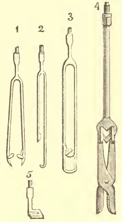
Tools for Extracting Obstructions.
